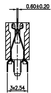
PLASTIC POST
